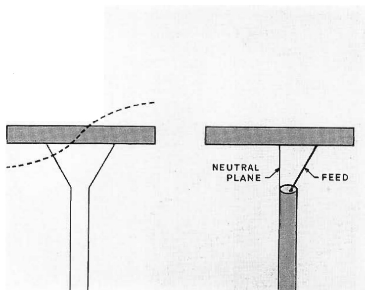
FIG. 13. The simple shunt feed system is based on the common delta-match principle.
