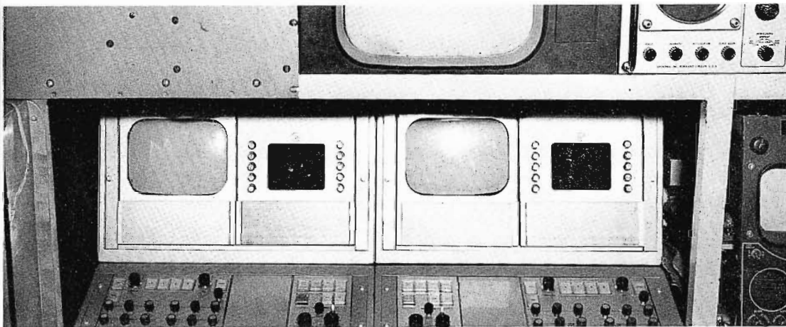
FIG. 6. RCA TK-42 color camera control consoles which are installed in KVVH-TV's mobile videotaping unit. This complete MVTR unit is connected into the KVVH studio control when not in use elsewhere, thus making the TK-42 cameras and their controls available for both remote and studio use.
