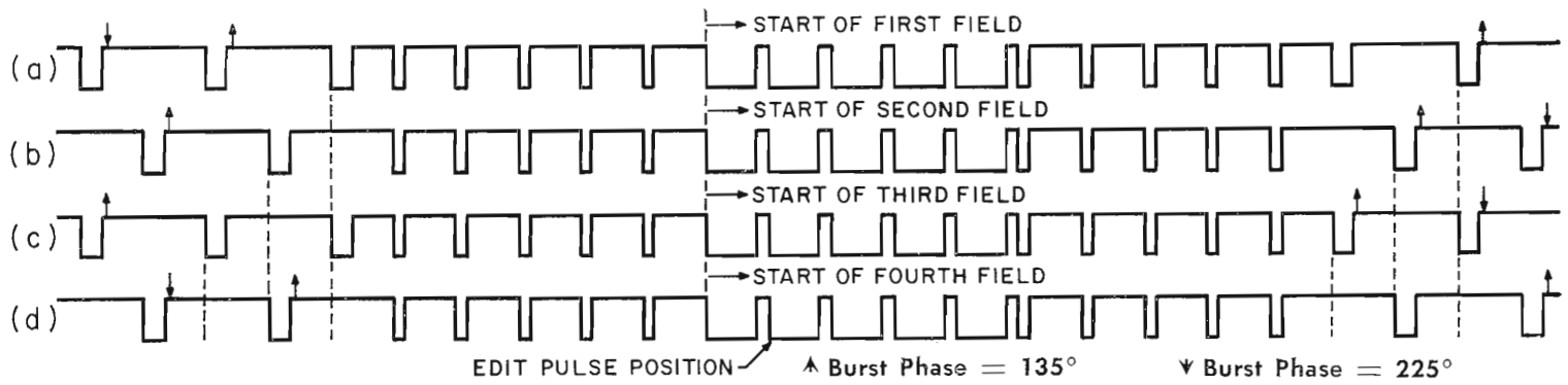
FIG. 8. Diagram showing PAL "meandering" burst repetition.
