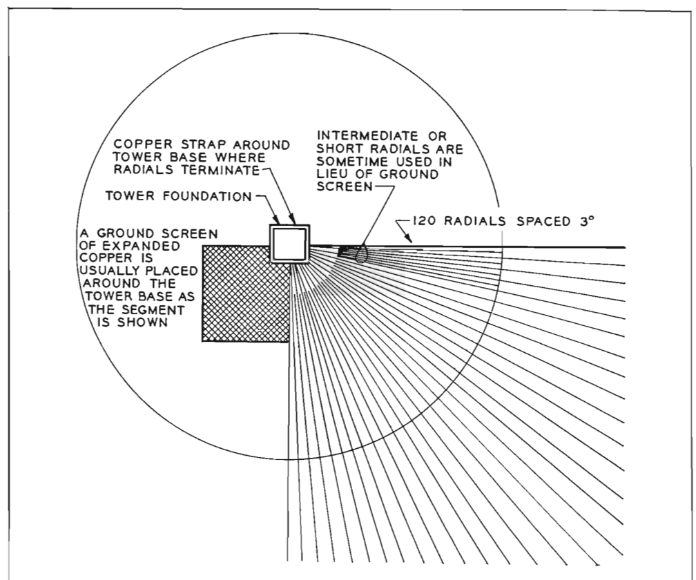
FIG. 10. Typical ground system. Radials and ground screen are positioned all the way around the tower base in each of the four quadrants as shown.
