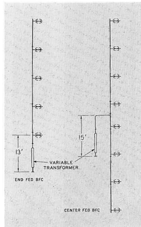
FIG. 19. BFC antenna feed systems.
