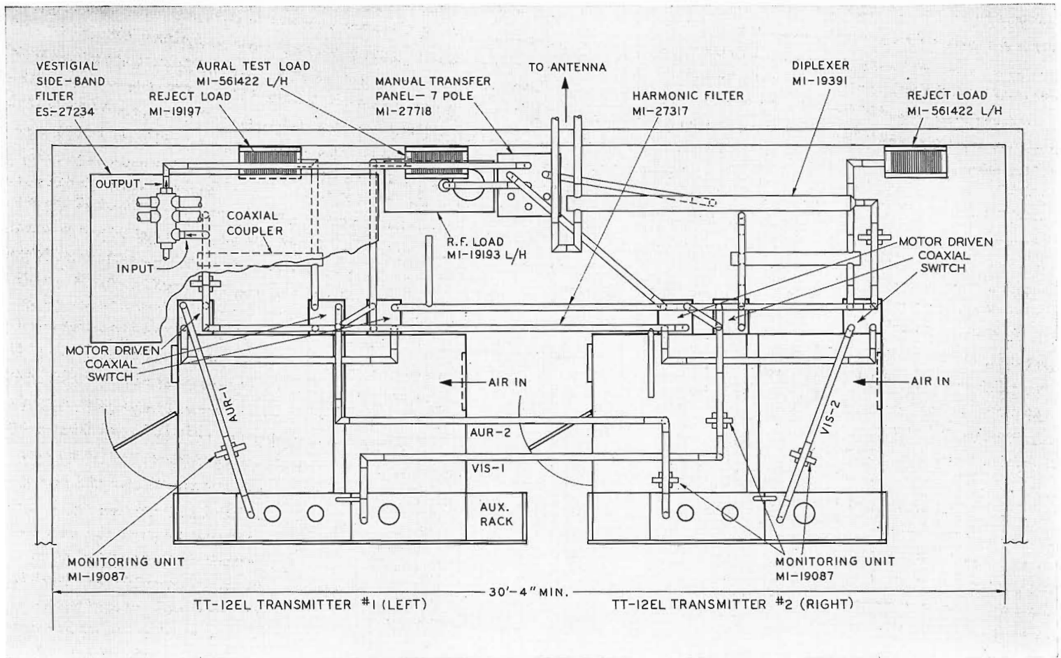
FIG. 3. A typical floor plan showing parallel operation of two TT-12EL Transmitters. The layout shows the coaxial switching system, aural and visual reject loads, diplexers and associated monitoring equipment.
