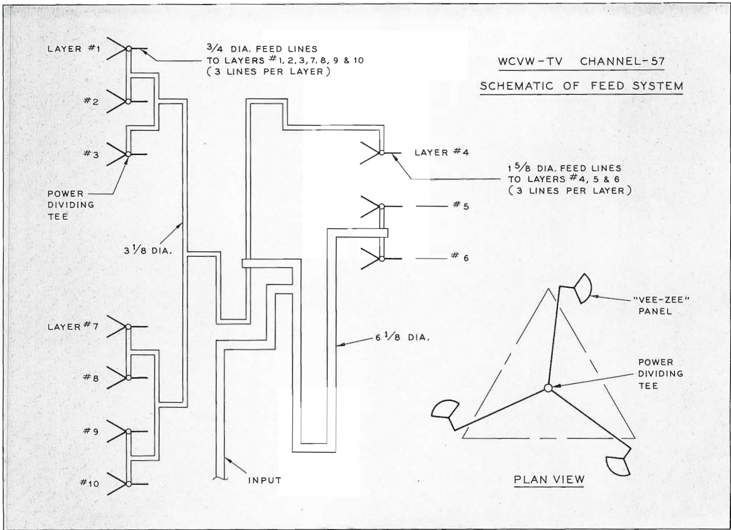
FIG. 11. Channel 57 "Vee-Zee" Panel Antenna feed system.
