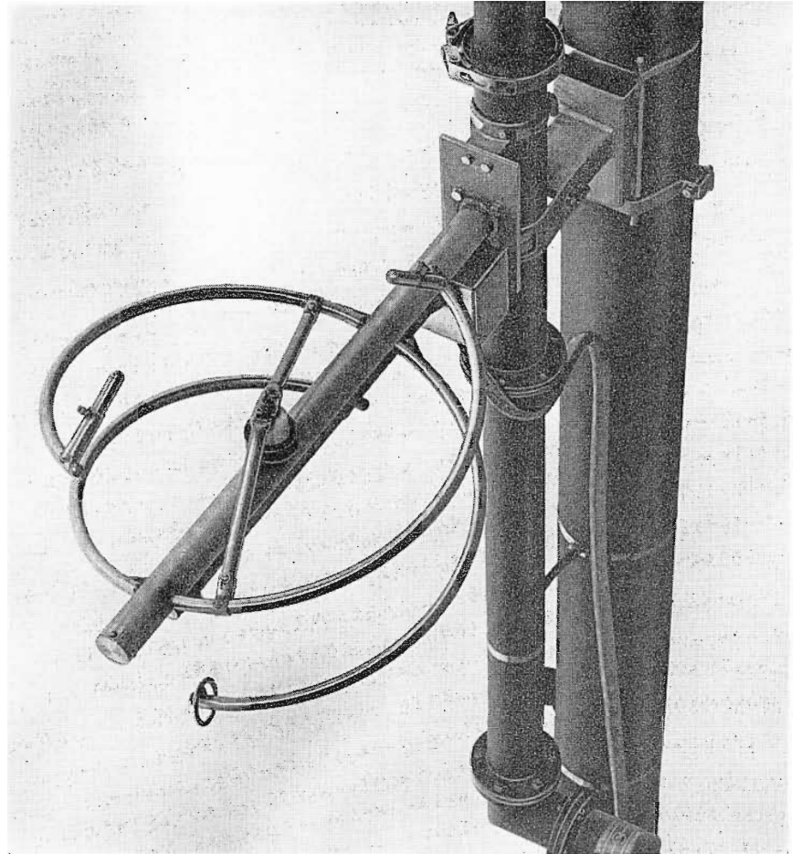
FIG. 2. BFC Circularly Polarized Antenna radiator.
