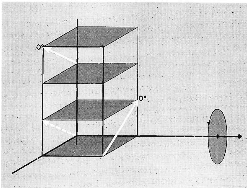
FIG. 9. Current elements of Fig. 8 each rotated and shifted in their respective planes still result in circularly polarized radiation in one direction.
