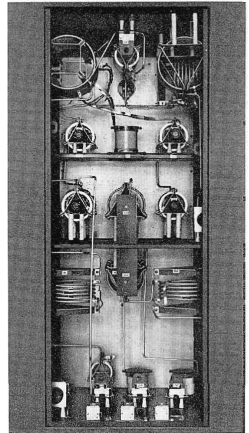
FIG. 9. Phasing equipment for a three-tower system.
