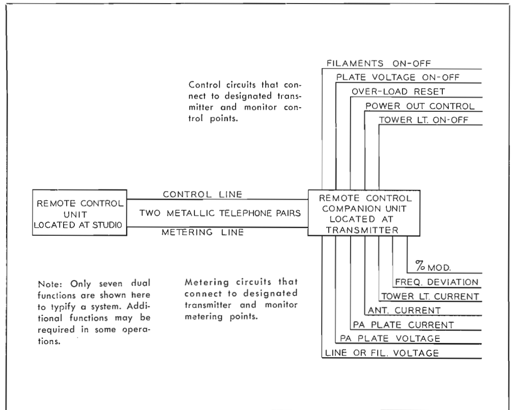
FIG. 23. Block diagram of typical remote control system. Two telephone lines are used between studio and transmitter, one for control, the other for monitoring. Additional functions may be added to system. Equipment is available to convert the BTR-20D to tone operation, permitting operation on a single voice-grade telephone line or microwave link.
