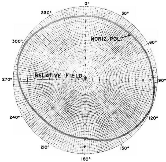
FIG. 14. Horizontal pattern of the horizontally polarized signal component in free space.
