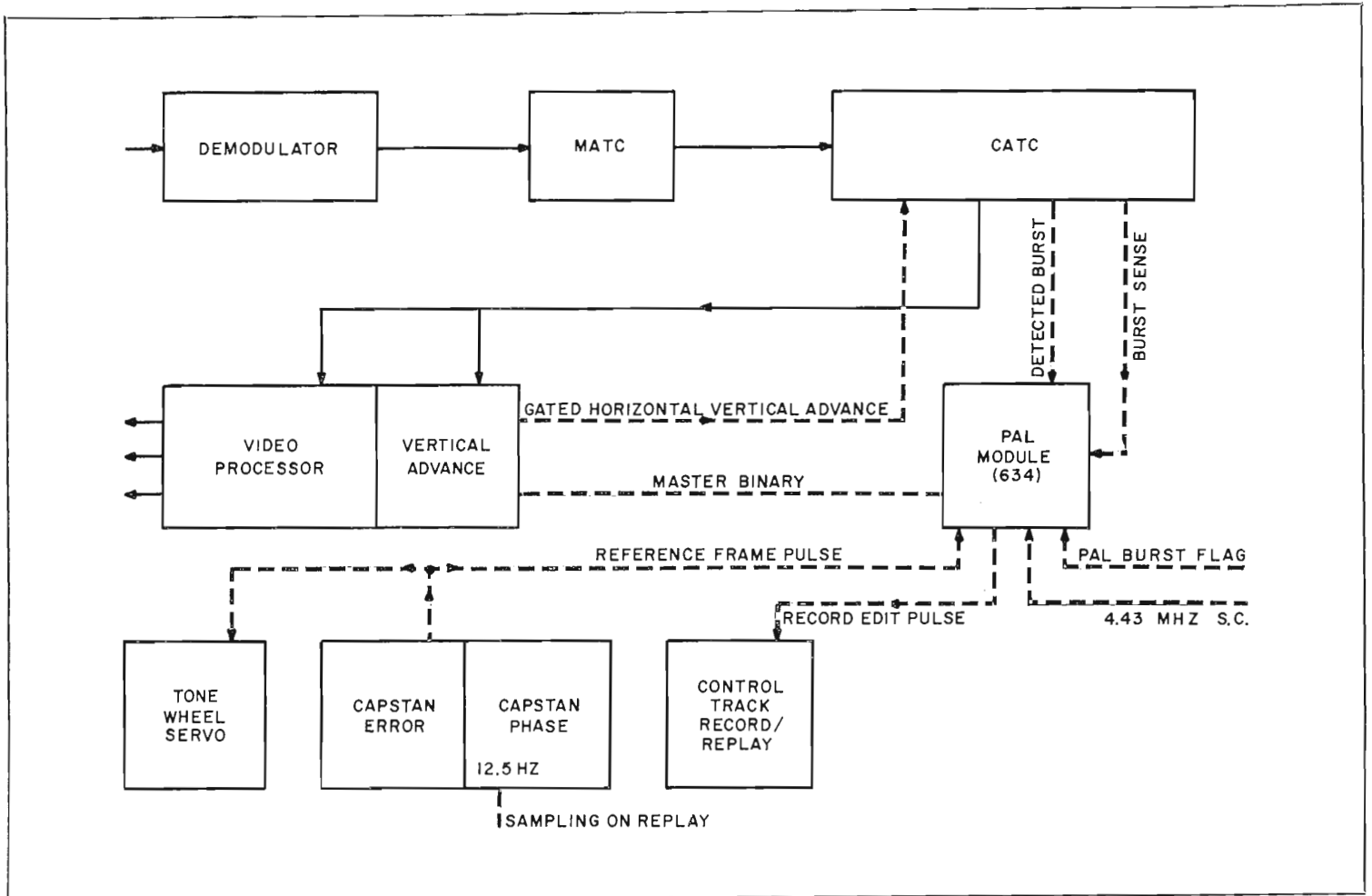
FIG. 7. Simplified block diagram showing elements of PAL circuitry in dashed lines.
