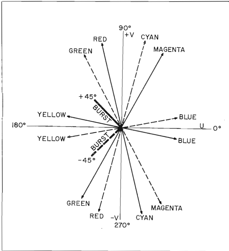
FIG. 3. PAL vector diagram for six colors.
