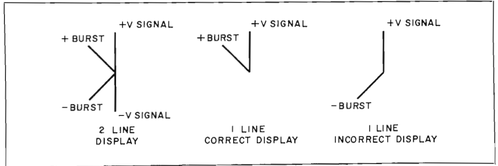
FIG. 5. Diagram showing burst switching requirements.
