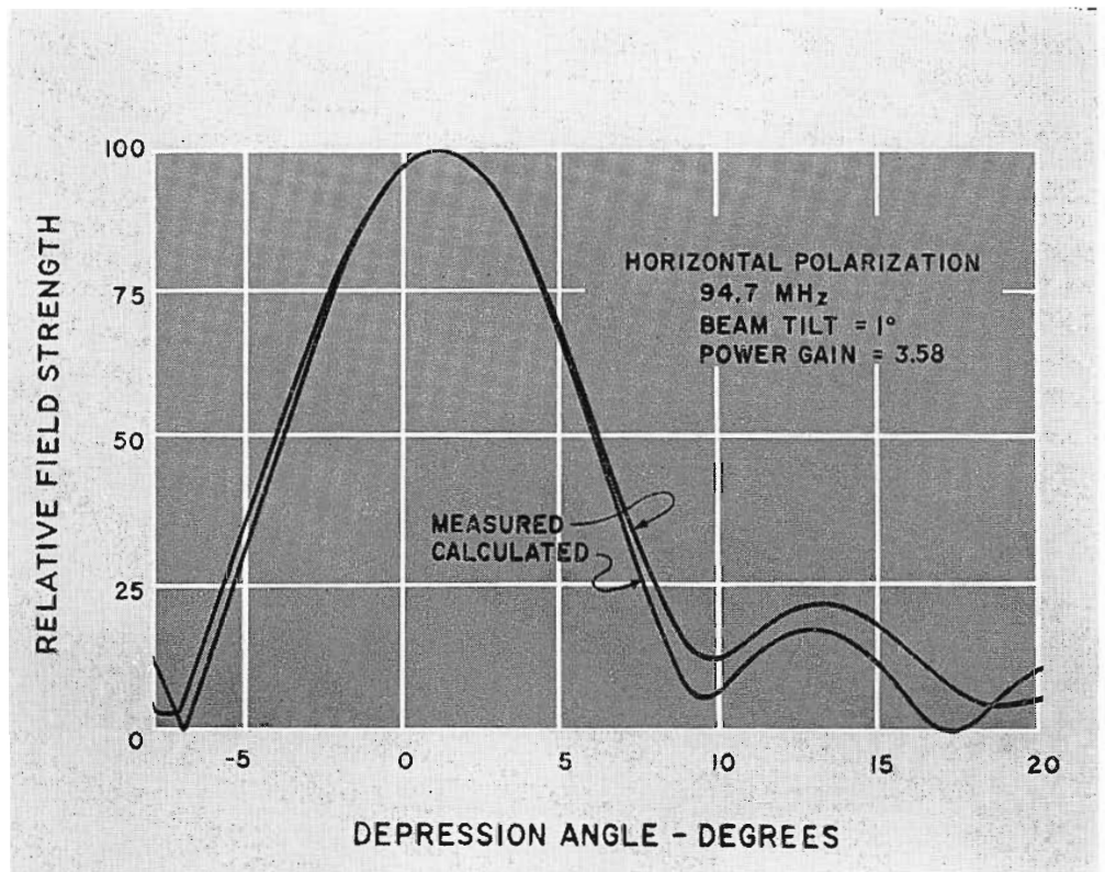
FIG. 16. Vertical radiation pattern of a BFC-7 antenna.
