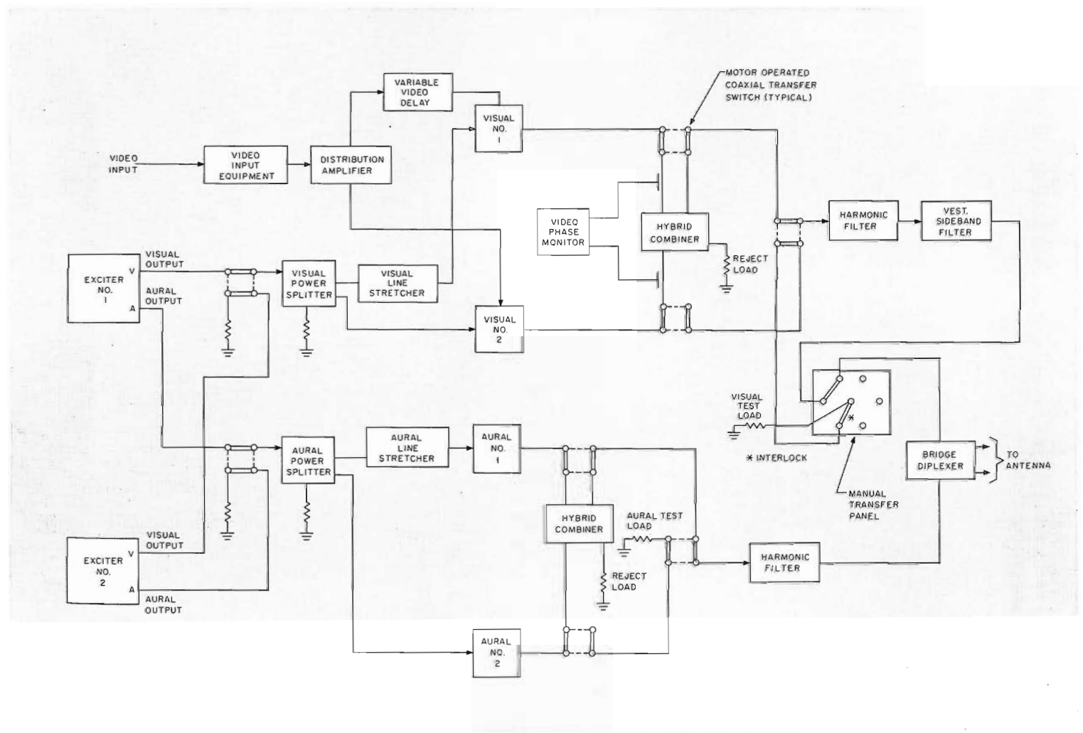
FIG. 5. Simplified block diagram of the TT-12/12EL parallel transmitter system. Switching arrangement permits the selection of either exciter unit and other RF circuits.
