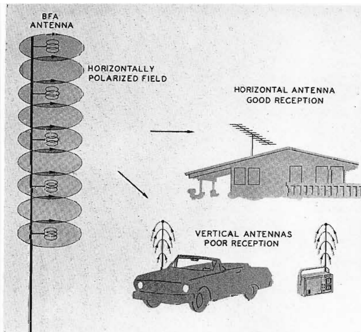
FIG. 3. Horizontally polarized transmission provides good reception for homes but tends to serve autos and portables poorly.
