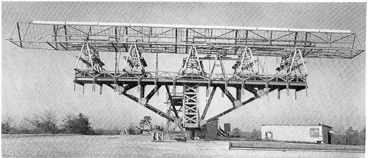
FIG. 10. Ten "Vee-Zee" panels stacked on one leg of simulated tower section, undergoing vertical pattern tests.
