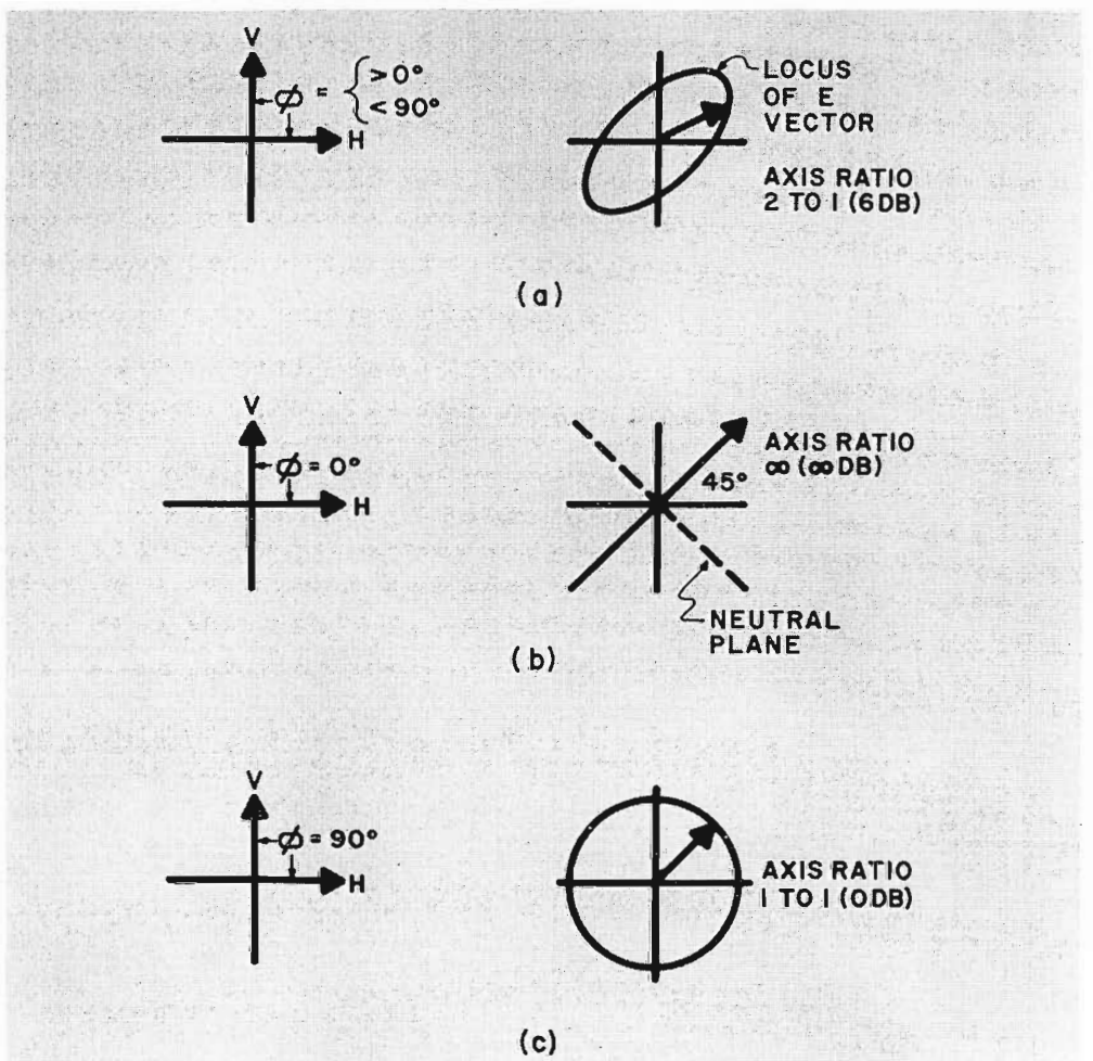
FIG. 6. Total fields produced by two orthogonal signals for elliptical polarization (a), linear polarization (b), and circular polarization (c).
