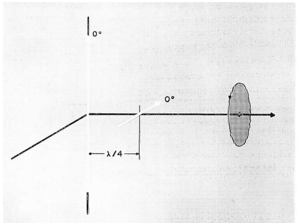
FIG. 8. The phase quadrature is produced by two in-phase current elements separated by a quarter wavelength.
