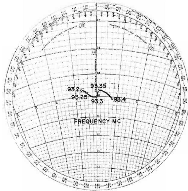
FIG. 18. Typical input impedance plot.
