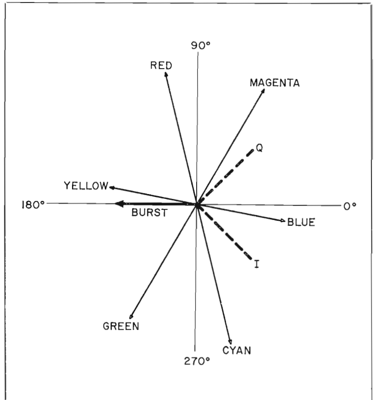
FIG. 4. NTSC vector diagram for six colors.
