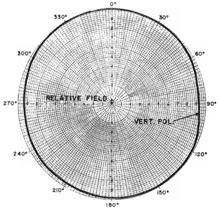
FIG. 15. Horizontal pattern of the vertically polarized signal component in free space.
