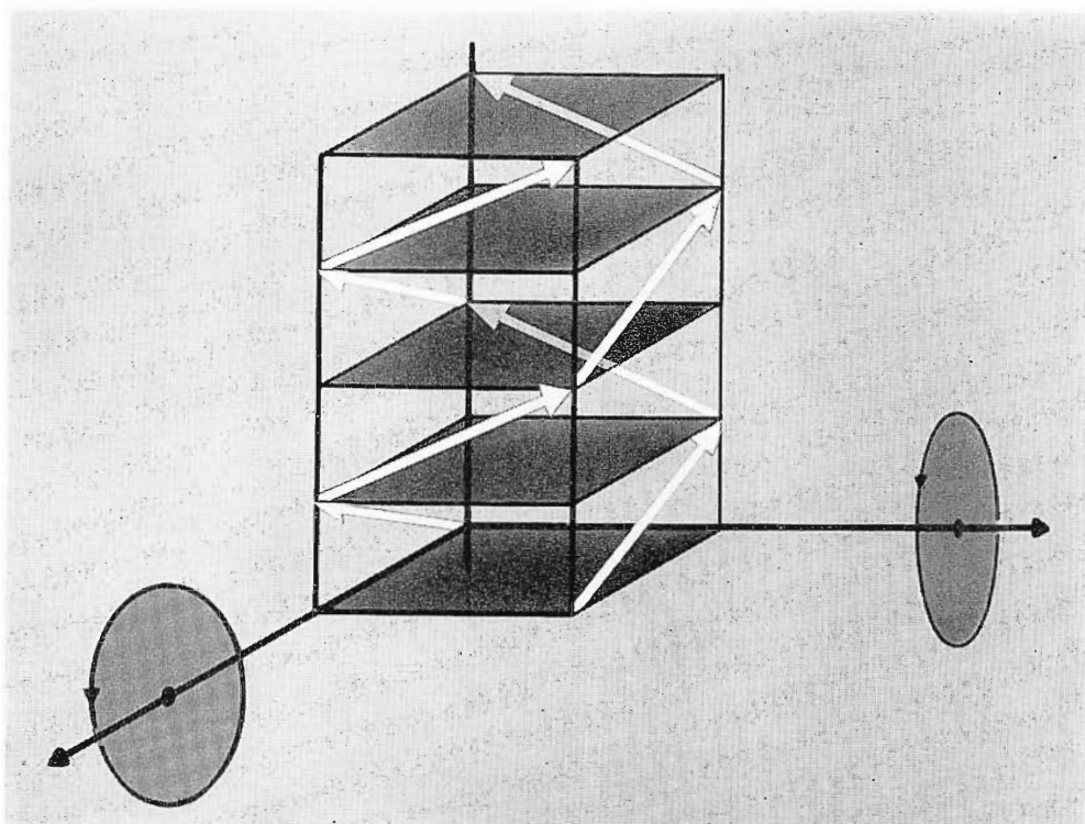
FIG. 11. Two resonant half wave dipoles are curved into one-turn helices each and interlaced to maintain constant current around as required for omnidirectional service. Thus, a practical broadband radiating element is obtained.
